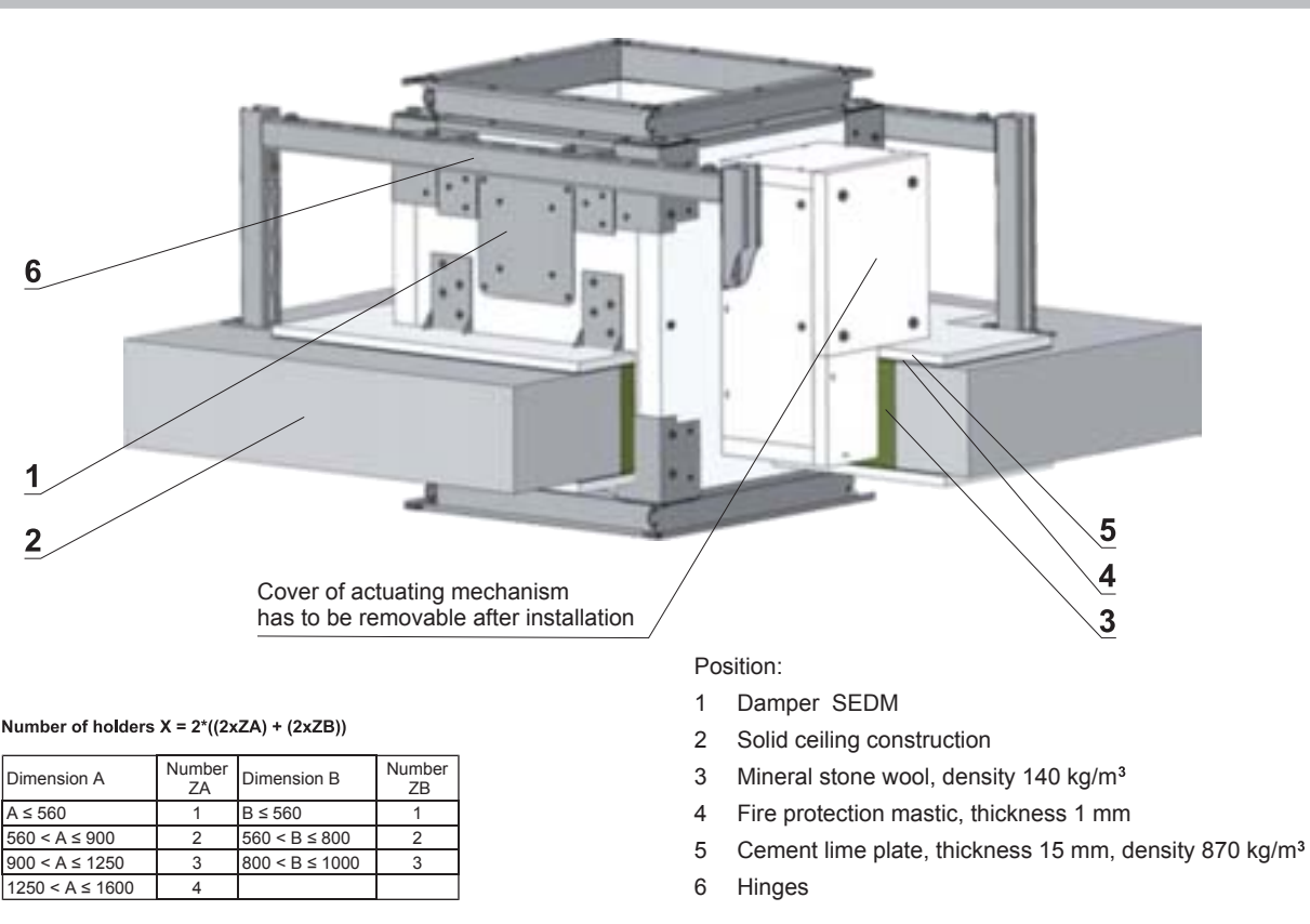
Fig. 24 Example of installation in solid ceiling construction of fire compartment - actuating mechanism above
