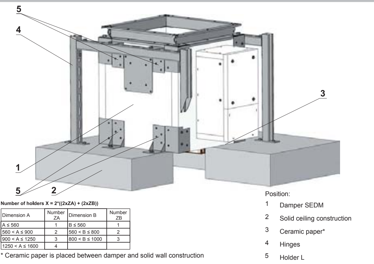
Fig. 36 Example of installation on solid ceiling construction of fire compartment - above installation.
