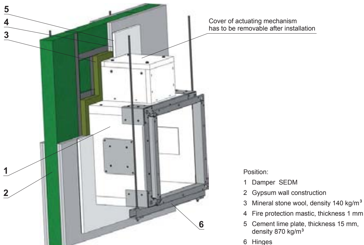
Fig. 29 Example of installation in gypsum wall construction of fire compartment.
