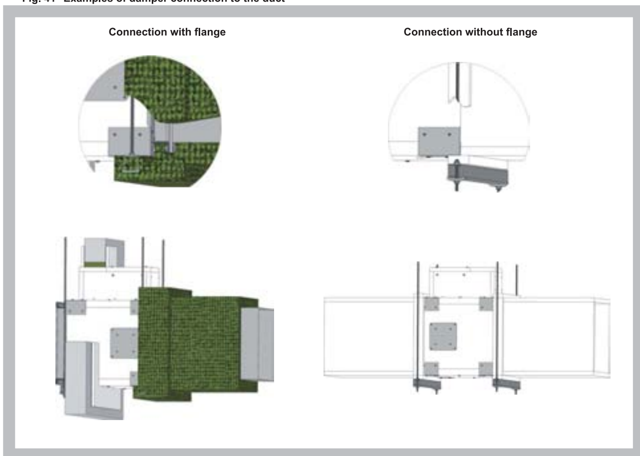
Fig. 41 Examples of damper connection to the duct
