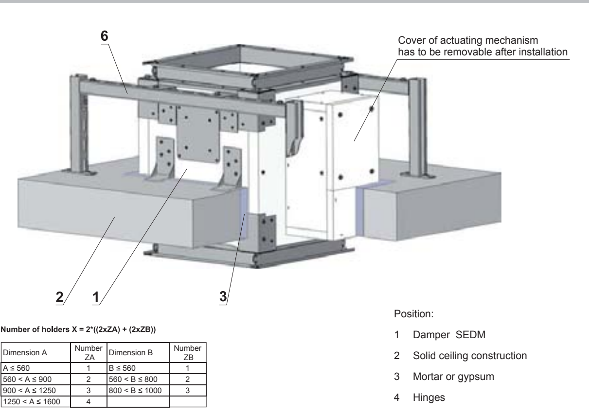
Fig. 26 Example of installation in solid ceiling construction of fire compartment - actuating mechanism above
