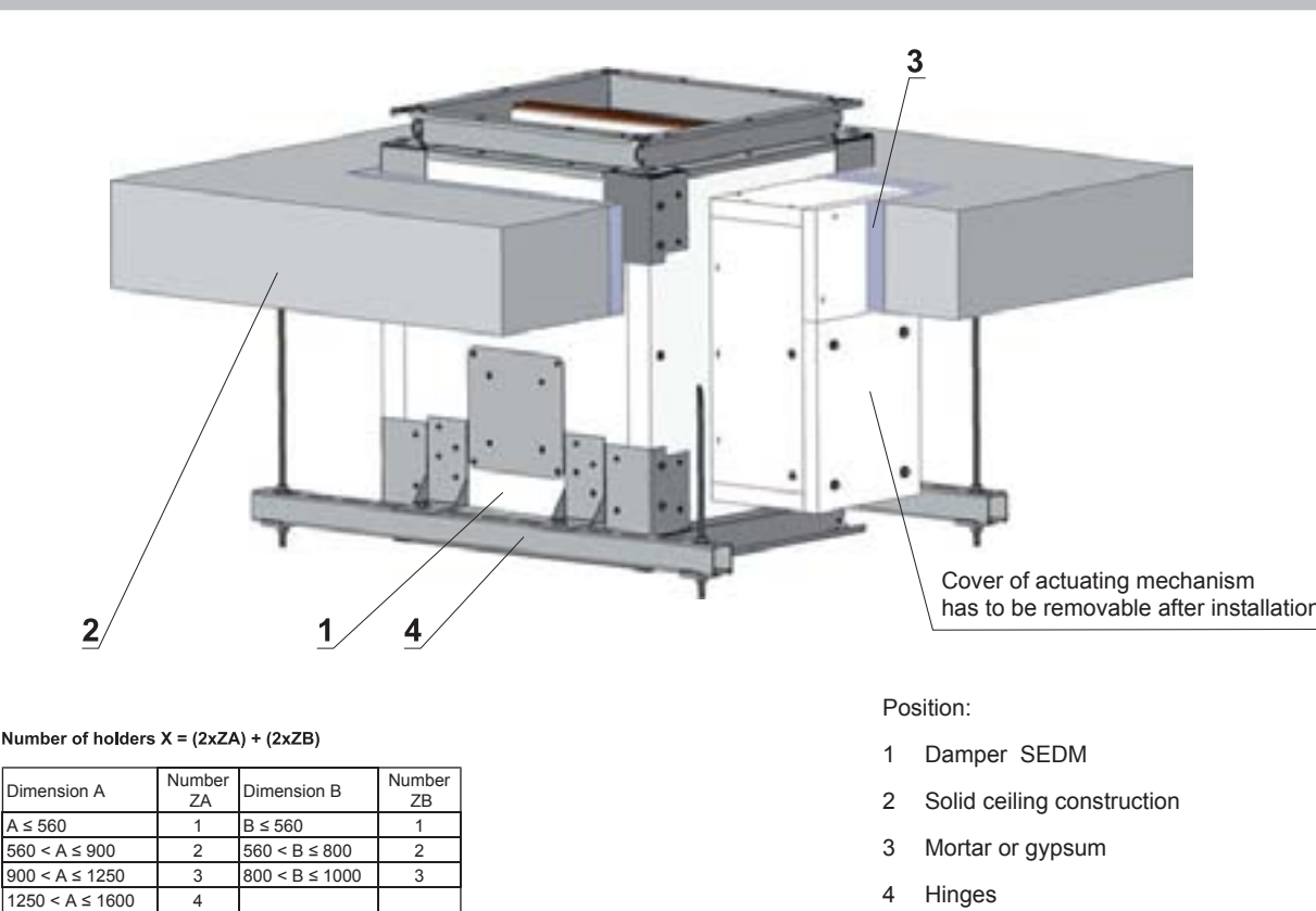
Fig. 25 Example of installation in solid ceiling construction of fire compartment - actuating mechanism below
