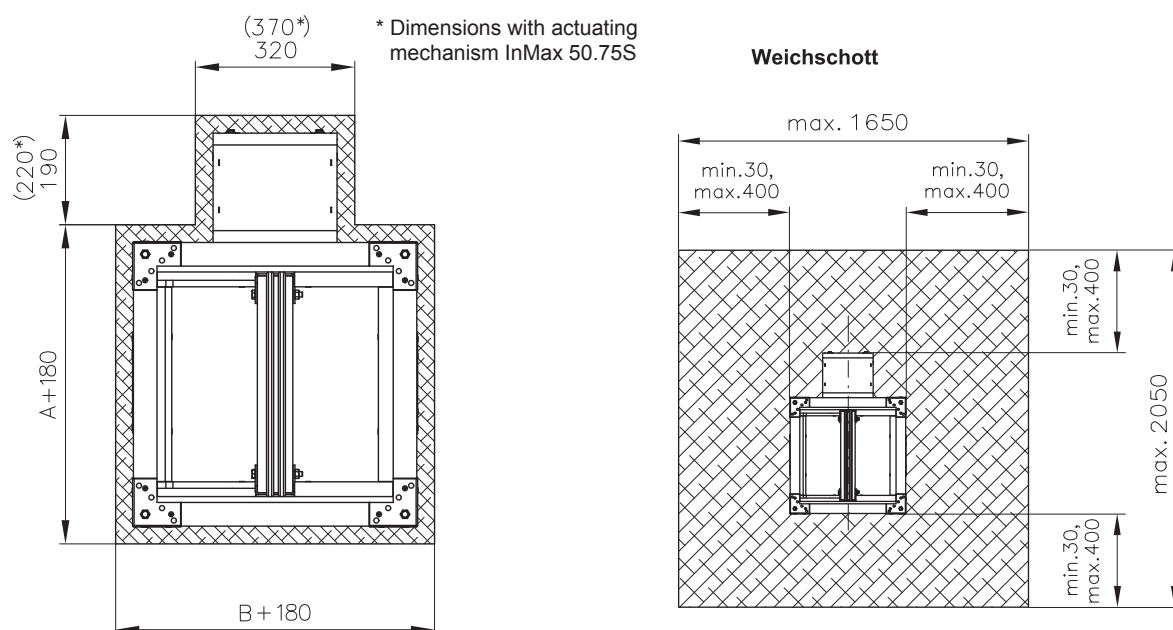
Fig. 13 Installation opening
