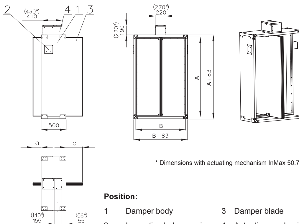
Fig. 11 Smoke extraction dampers - multi without flanges
