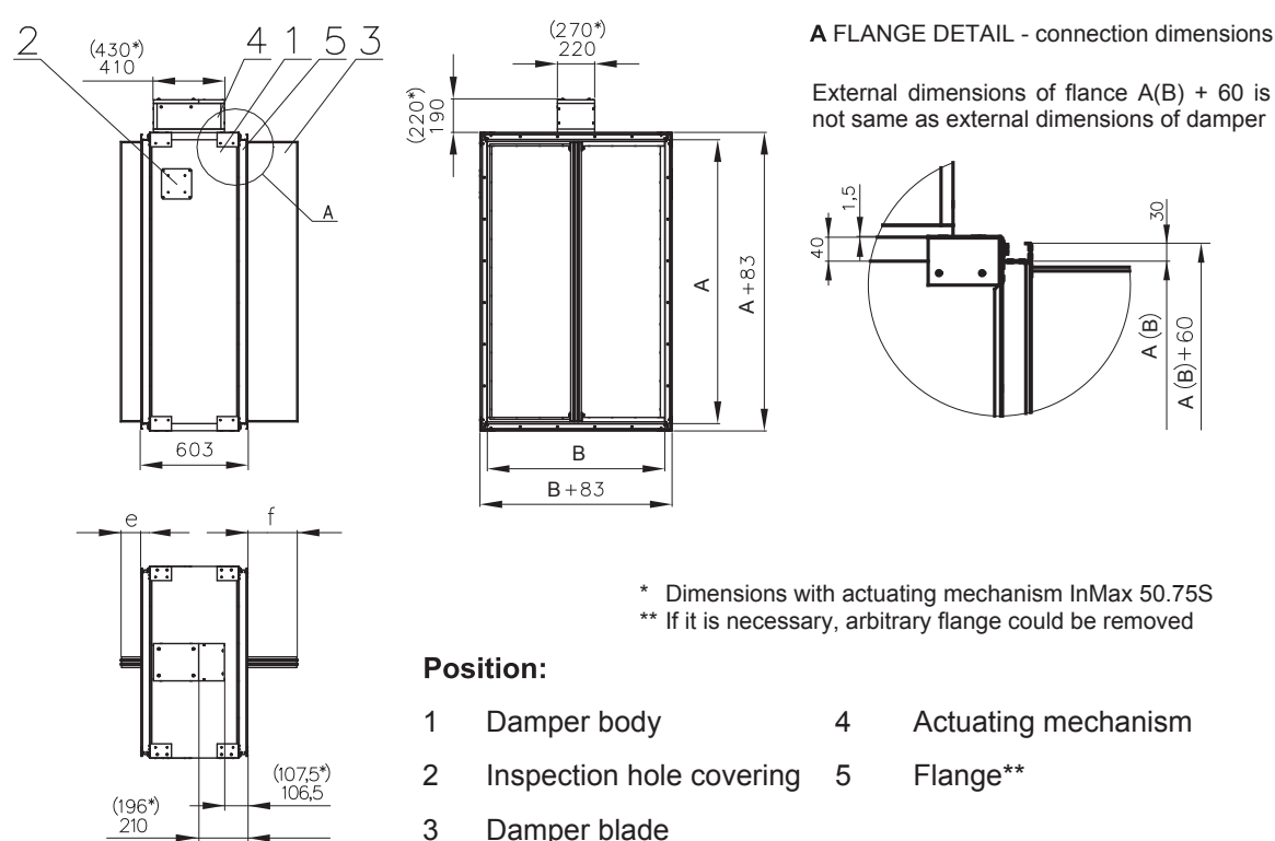
Fig. 12 Smoke extraction dampers - multi with flanges
