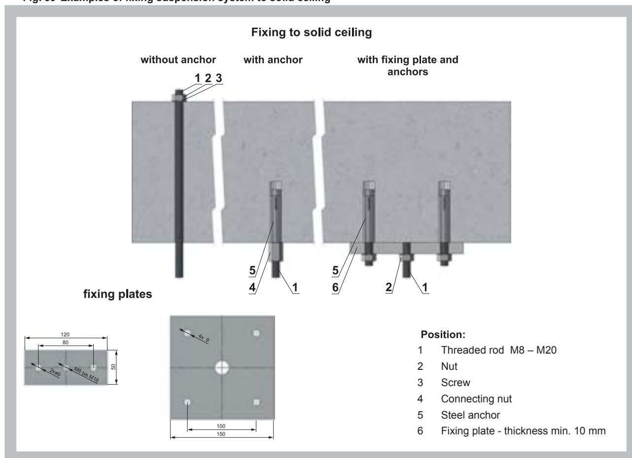
Fig. 39 Examples of fixing suspension system to solid ceiling
