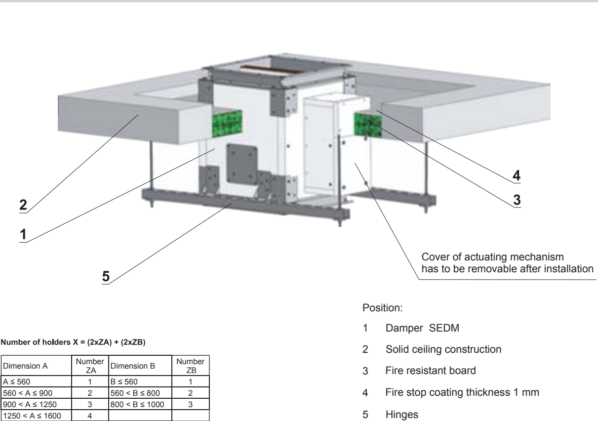
Fig. 27 Example of installation in solid ceiling construction of fire compartment - actuating mechanism below
