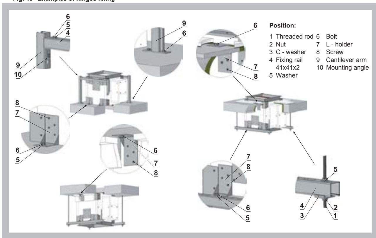
Fig. 40 Examples of hinges fixing
