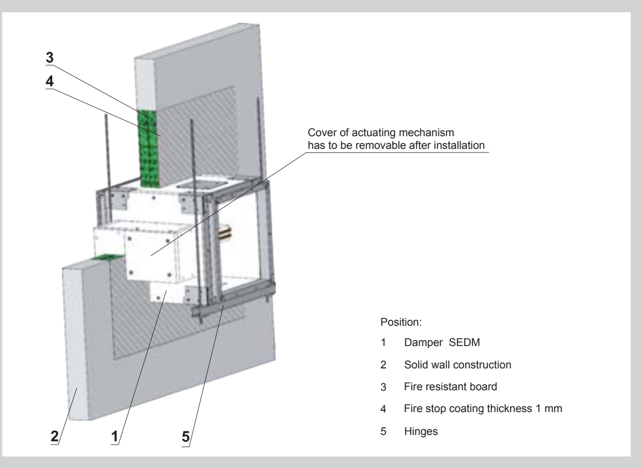
Fig. 22 Example of installation in solid wall construction of fire compartment - horizontal blade axis position.
