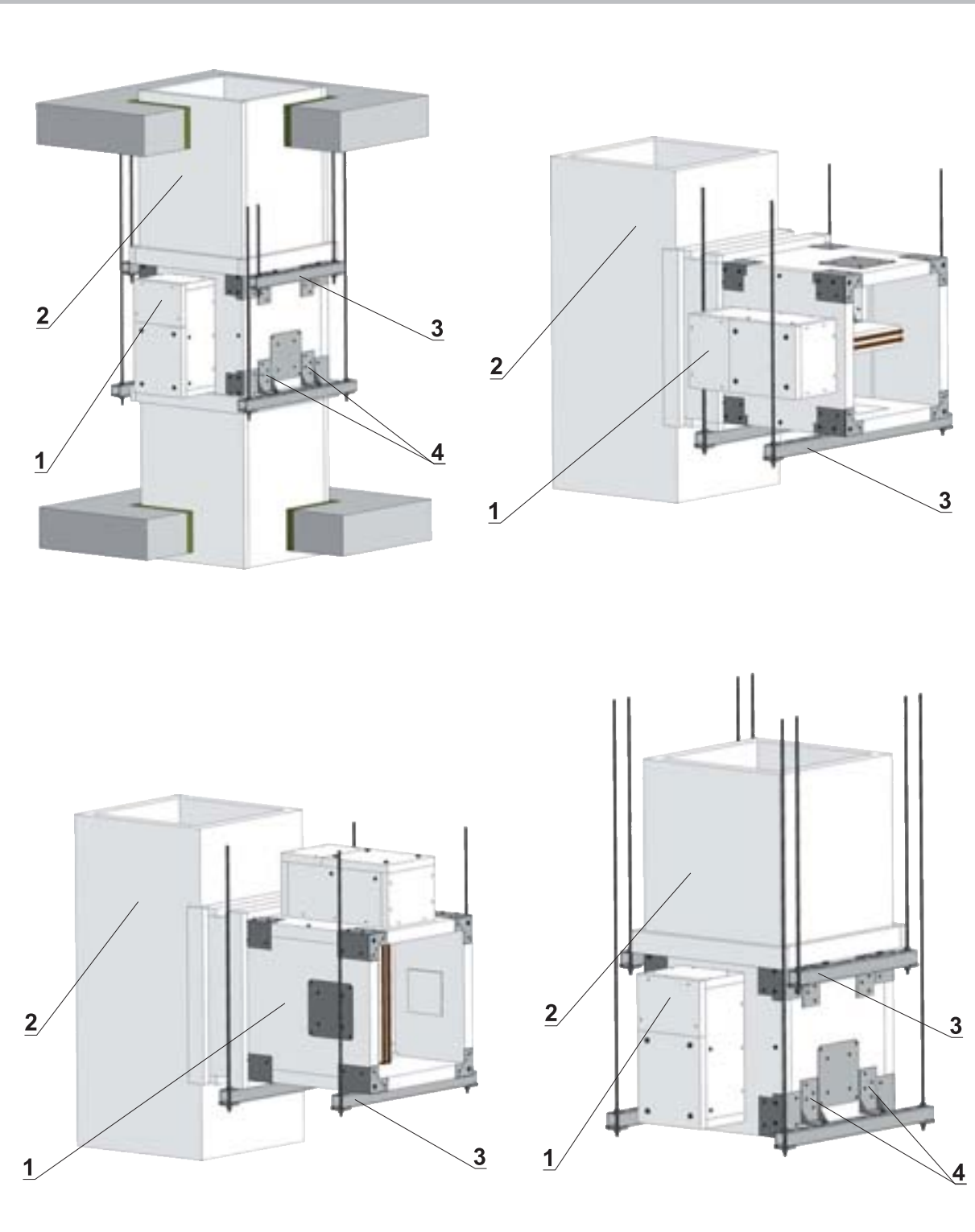
Fig. 37 Example of installation in vertical smoke exhaust duct.
