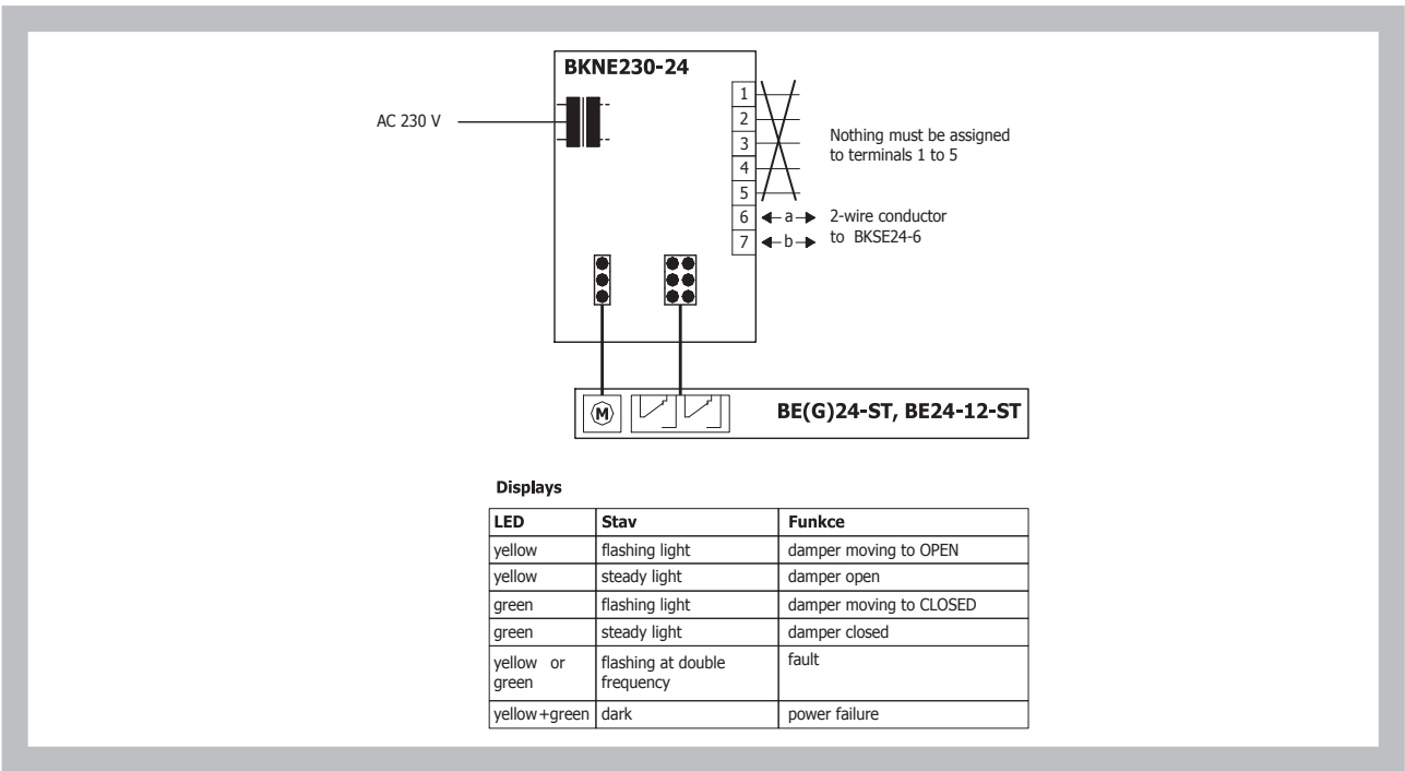
Fig. 9 Communication and supply device BKNE 230-24
