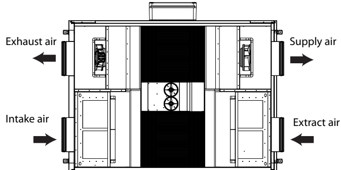
Right-sided modification (top view)
