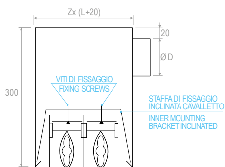
Fissaggio al plenum con staffe inclinate CVL cavalletti Fixing to the plenum by inner mounting brackets inclined CVL
