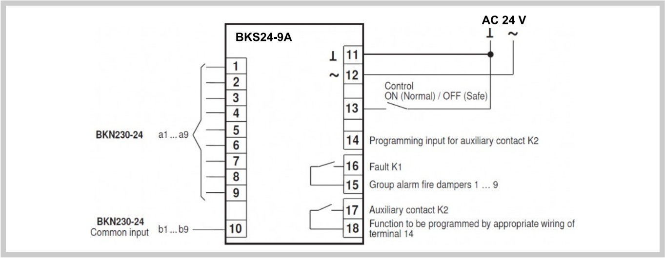
Wiring diagram BKS24-9A
